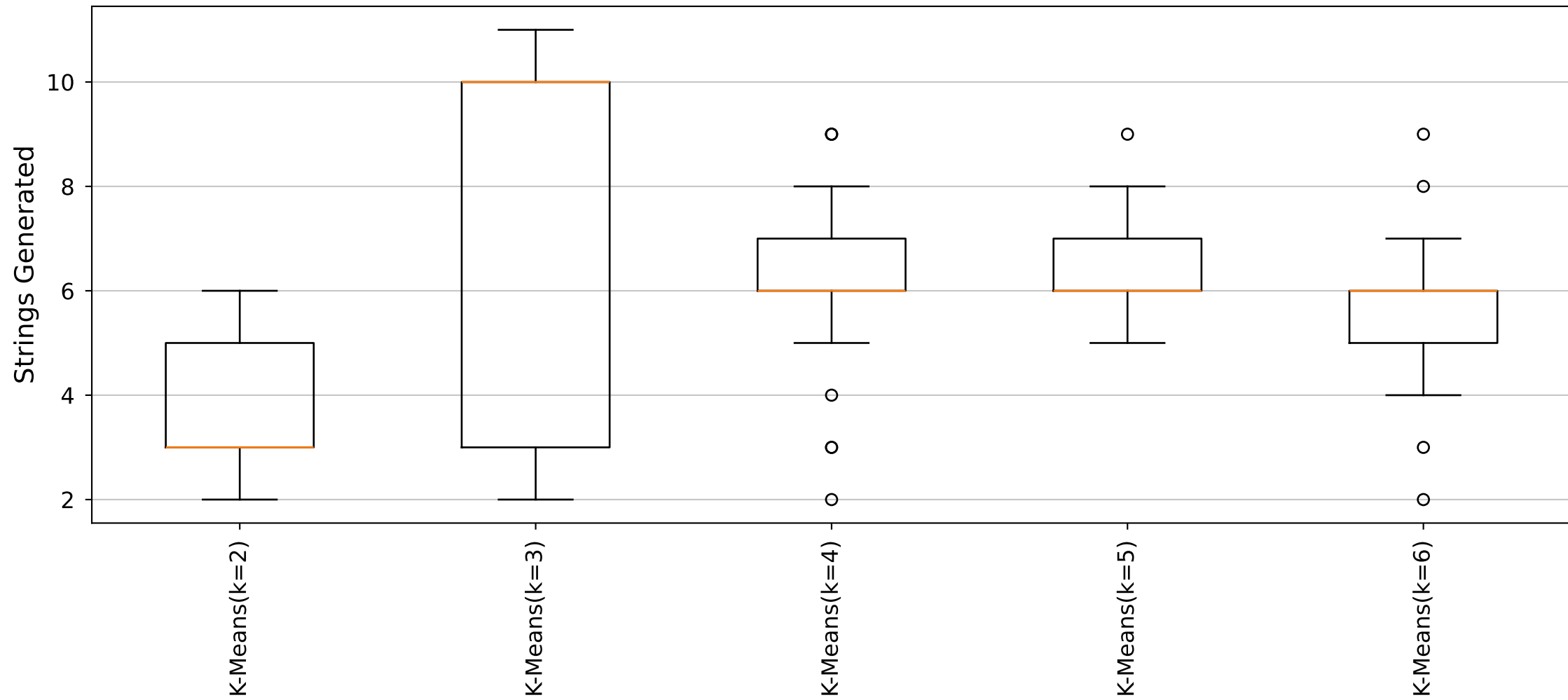
YARA Rules Strings Generated Distribution (Cluster32_Size6 dataset)
